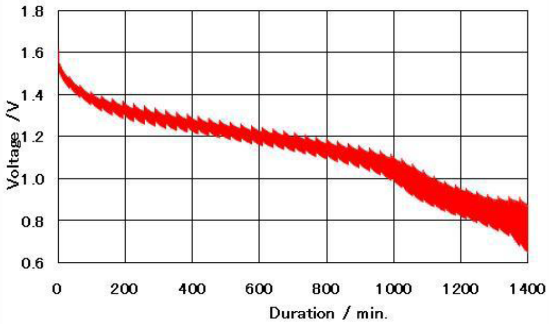
Portable Light : 3.9 \Omega 4min. on/56min. off 8H/D
